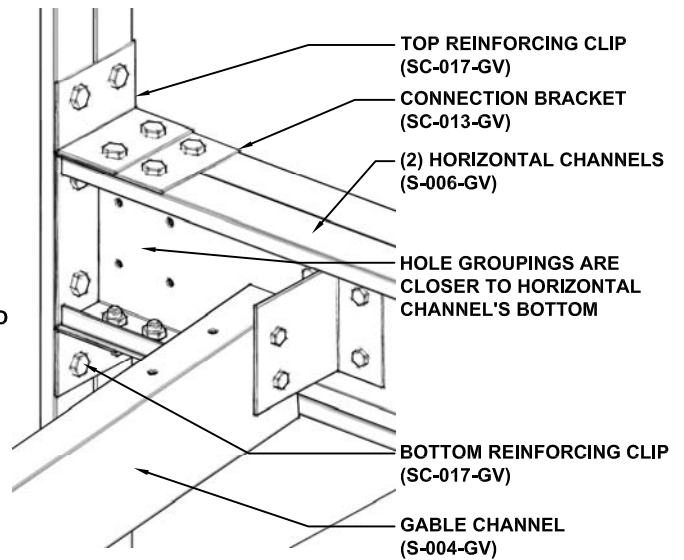
FIGURE 9 - INTERIOR SUPPORT
